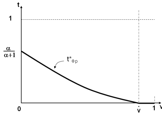
Figure 3a c = 0
