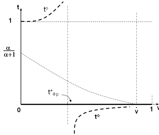
Figure 3c c > \alpha\dot{v}/4
