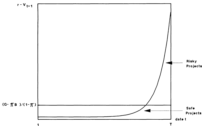
FIG. 4.—The time series of r_t - V_{t+1} assuming f_B = 0 . Assuming that f_B = 0 implies that interest rates are constant at the riskless rate, i.e., r_t = r .
